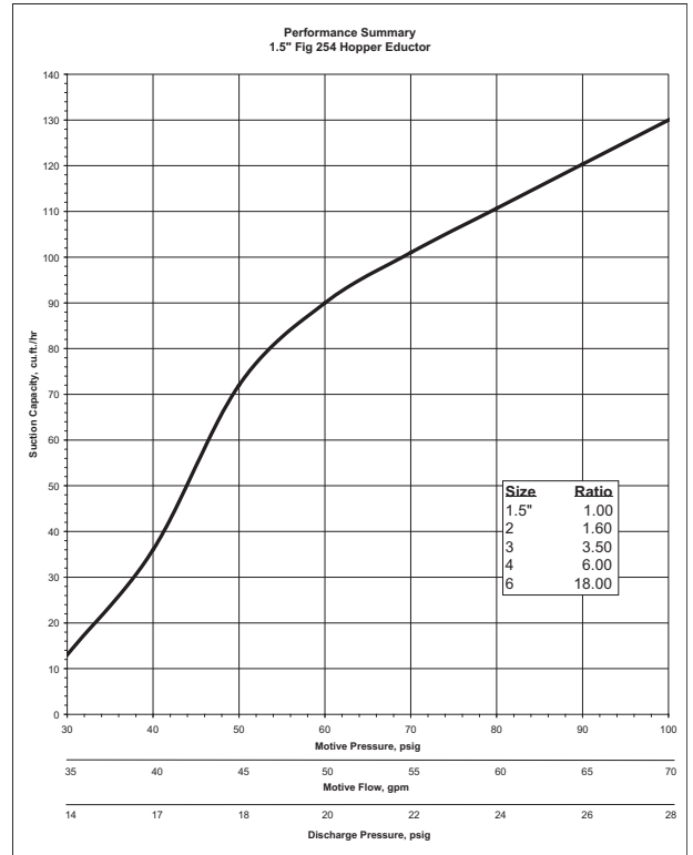
Chart 254. Performance Summary of 1 1/2" Hopper-Equipped Eductor, Fig. 254.
