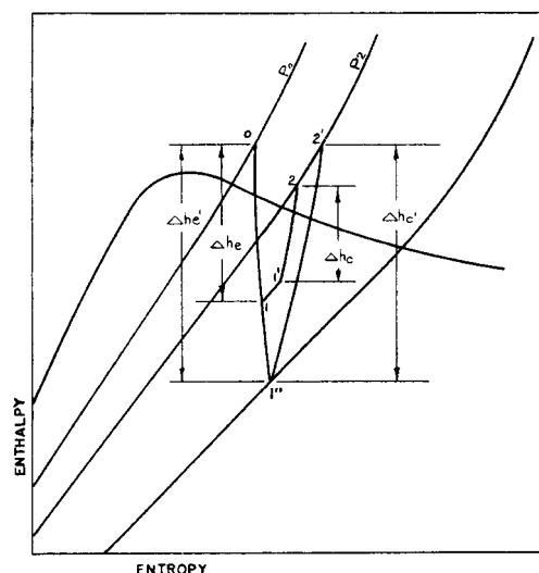
Fig. 2 Typical thermodynamic cycle for steam jet-vacuum pump operating with a suction load (0-1-2), and at zero suction load (shutoff) (0-1'-2')
