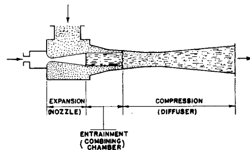
Fig. 1 Fundamental steam jet-vacuum pump parts
