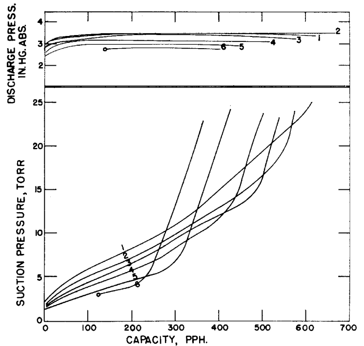
Fig. 6 Typical effect of nozzle location on stage performance
