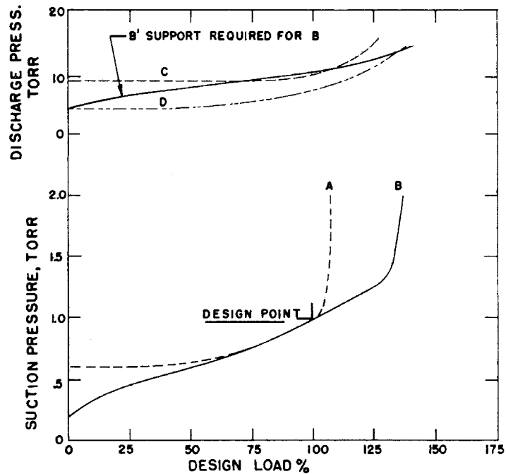
Fig. 10 Typical combination of two noncondensing stages
