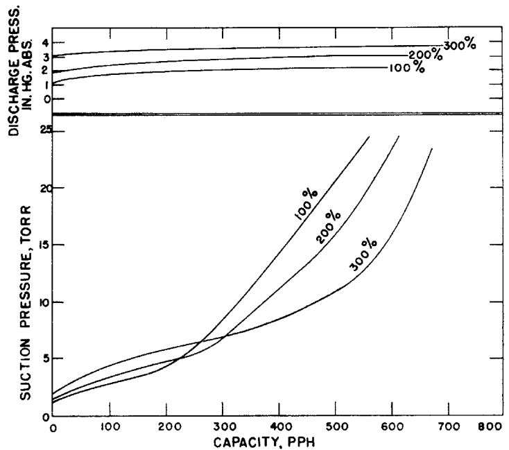
Fig. 7 Typical effect of steam rates on stage performance
