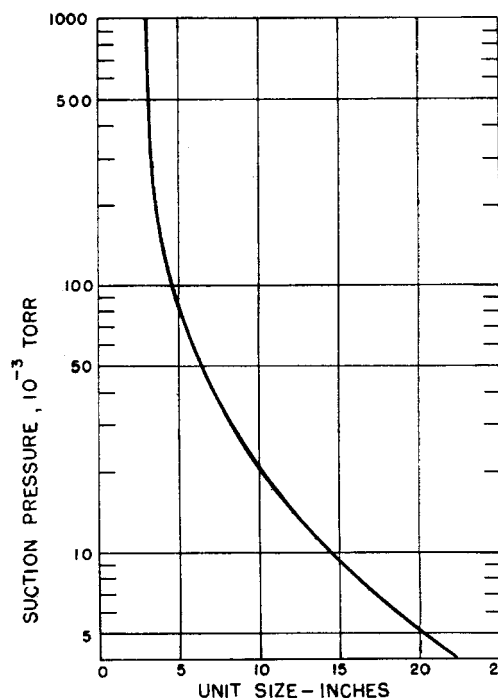
Fig. 9 Smallest practical stage size
