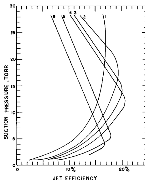
Fig. 8 Typical effect of nozzle position upon jet efficiency of one stage
