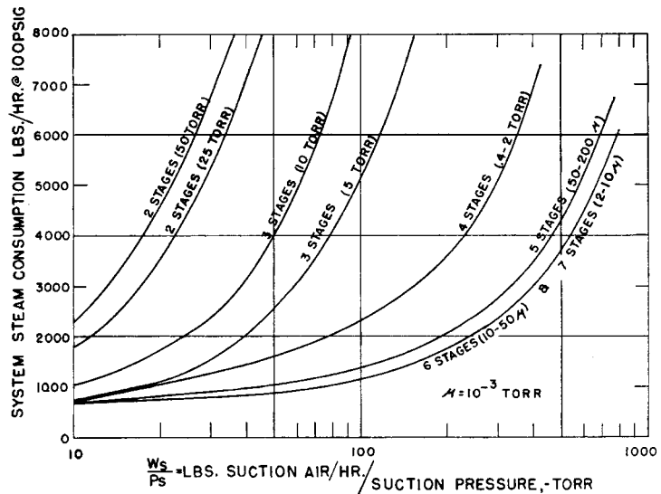
Fig. 11 Multistage, barometric condensing steam-jet vacuum pumps. Pumping and steam consumption characteristics at 100 psig steam, 85 F water, for air.
