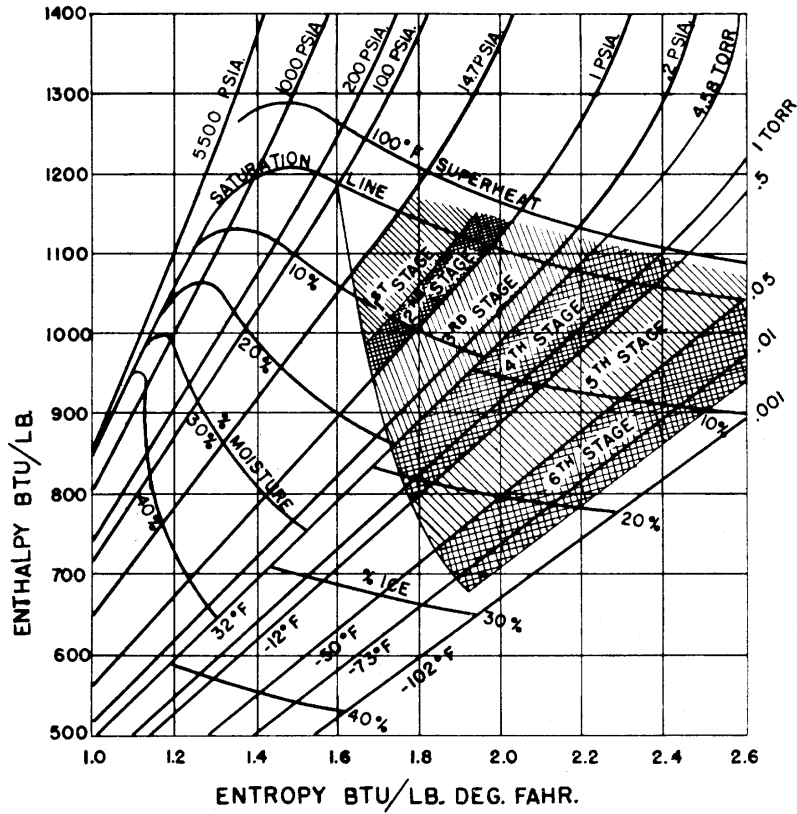
Fig. 3 Mollier diagram to 10^{-3} torr showing operating regions of steam jet-vacuum pump stages
