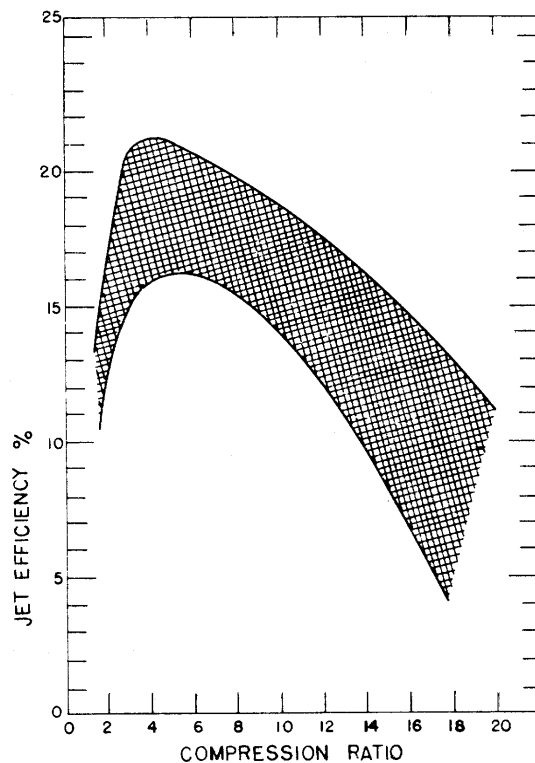
Fig. 5 Range of attainable jet efficiencies for steam-jet pumping air
