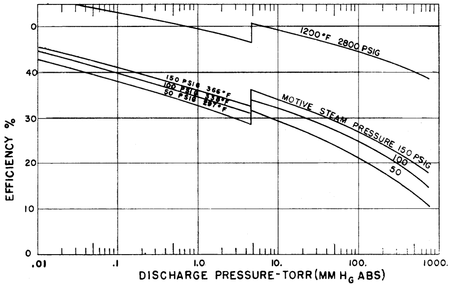
Fig. 4 Rankine cycle efficiency, steam jet-vacuum pump single stage
