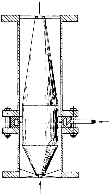
Fig. 8 Annular venturi-orifice desuperheater
