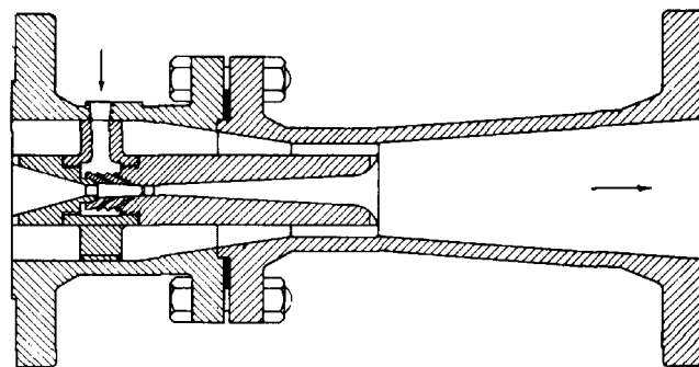
Fig. 1 Venturi desuperheater
