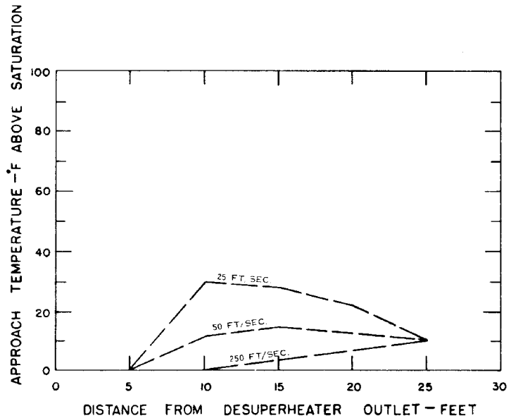
Fig. 4 Venturi desuperheater pipeline temperature gradients at various pipeline velocities
