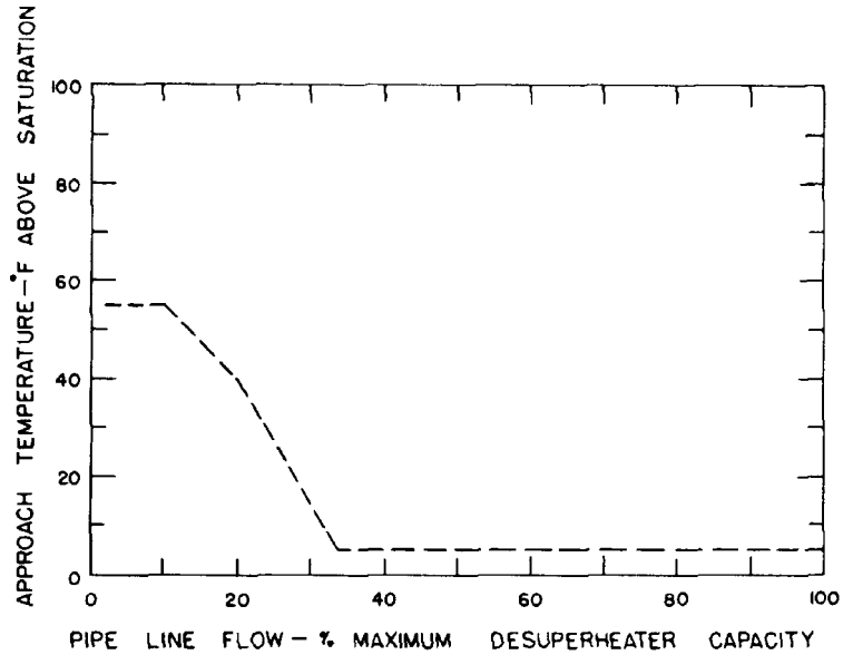
Fig. 7 Performance characteristics of steam ejector-atomizing desuperheater without recycle well, with atomizing steam pressure ratio of 2
