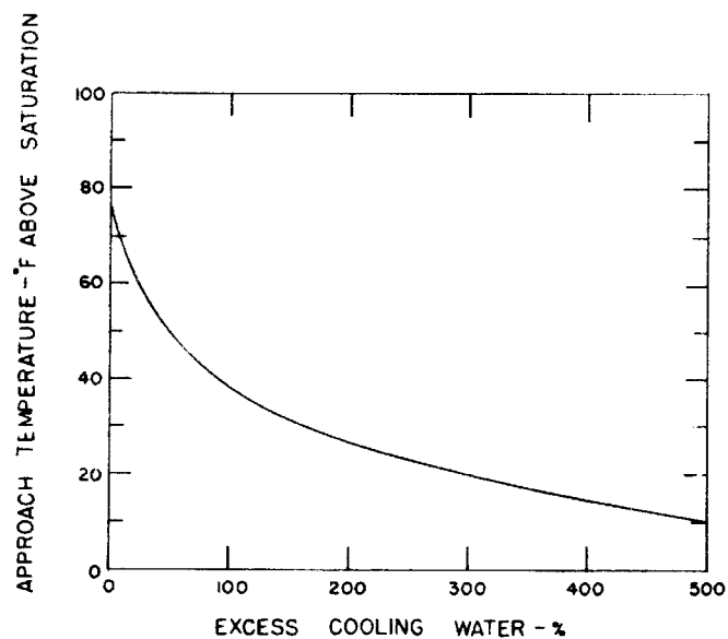
Fig. 3 Performance of a venturi desuperheater at 10 percent flow capacity with excess cooling water
