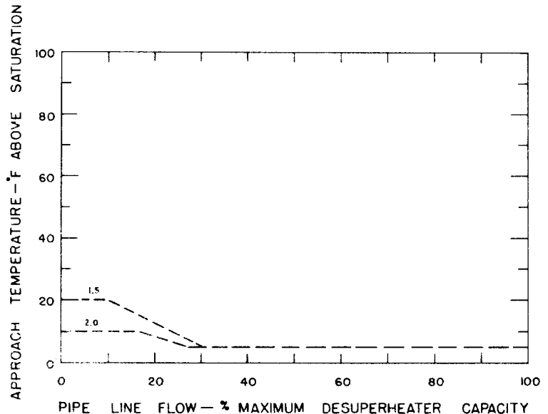
Fig. 6 Performance characteristics of recycle steam ejector-atomizing desuperheater at atomizing steam pressure ratios of 2 and 1.5
