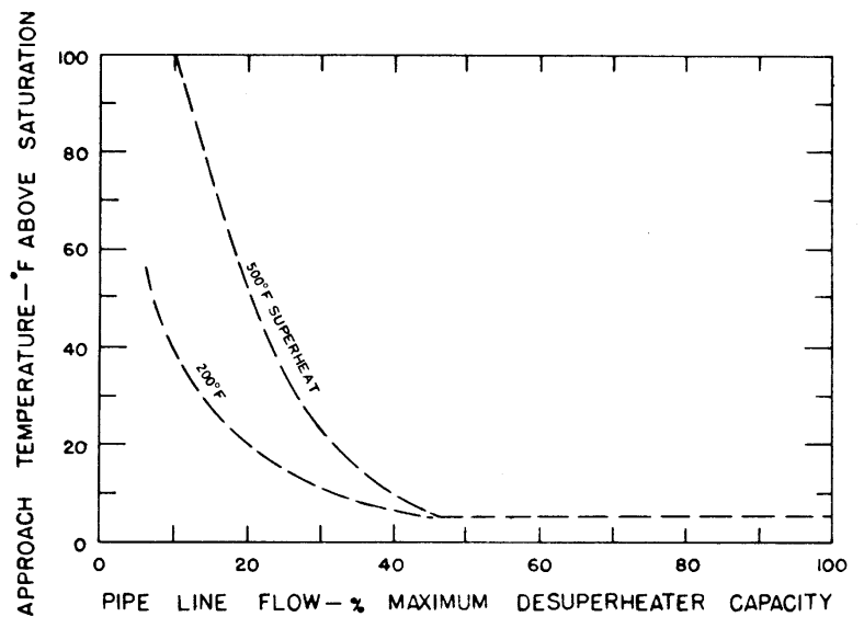
Fig. 2 Typical performance curves for a venturi desuperheater with no excess cooling water
