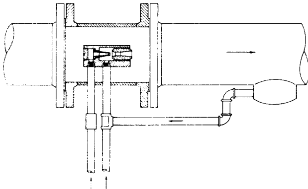
Fig. 5 Recycle steam ejector-atomizing desuperheater
